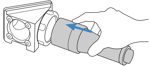
2 Insert the front part of the telecentric lens into port A of the CMMR
